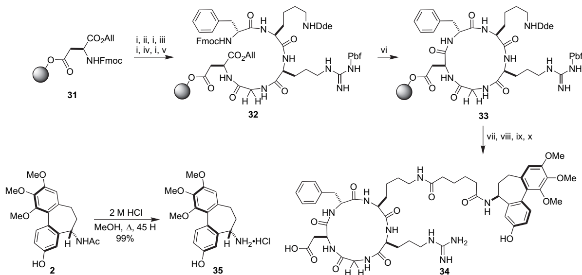
Scheme 7. Reagents and conditions: (i) piperidine–DMF (1:4), rt, 10 min ( \times 2 ); (ii) N - \alpha -Fmoc–Gly–OH (2 equiv), HCTU (2 equiv), DIPEA (4 equiv), DMF, rt, 2 h ( \times 2 ); (iii) N - \alpha -Fmoc–Arg(Pbf)–OH (2 equiv), HCTU (2 equiv), DIPEA (4 equiv), DMF, rt, 2 h ( \times 2 ); (iv) N - \alpha -Lys(Dde)–OH, HCTU (2 equiv), DIPEA (4 equiv), DMF, rt, 2 h ( \times 2 ); (v) N - \alpha -Fmoc–Phe–OH (2 equiv), HCTU (2 equiv), DIPEA (4 equiv), DMF, rt, 2 h ( \times 2 ); (vi) Pd(PPh 3 ) 4 (0.3 equiv), CHCl 3 –AcOH– N -methylmorpholine (37:2:1), rt, 4 h; then piperidine–DMF (1:4), rt, 10 min; then HCTU (3 equiv), DIPEA (10 equiv), DMF, rt, 24 h; (vii) H 2 N–NH 2 ·H 2 O, DMF, rt, 5 min ( \times 2 ); (viii) adipic anhydride (10 equiv), DIPEA (12 equiv), rt, 20 h; (ix) colchicinol·HCl (3 equiv), HCTU (3 equiv), HOBt (3 equiv), DIPEA (6 equiv), DMF, rt, 60 h; (x) TFA–( i -Pr) 3 SiH–H 2 O (95:2.5:2.5), rt, 1 h. HCTU=2-(6-chloro-1 H -benzotriazole-1-yl)-1,1,3,3-tetramethyluronium hexafluorophosphate, HOBt=1-hydroxybenzotriazole, Dde=2-(4,4-dimethyl-2,6-dioxocyclohex-1-ylidene)ethyl, Pbf=2,2,4,6,7-pentamethyl-dihydrobenzofuran-5-sulfonyl.
